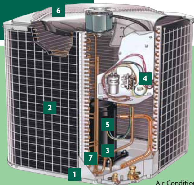
Air Conditioner
