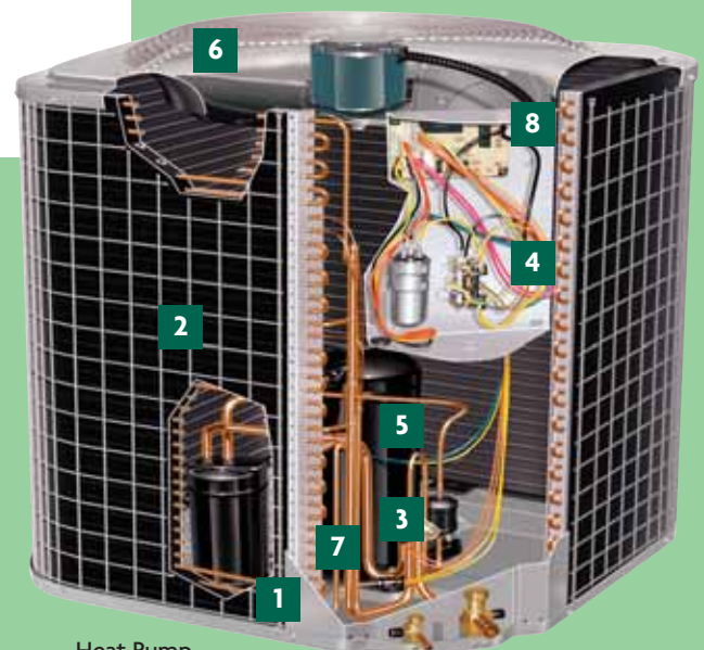
Heat Pump
