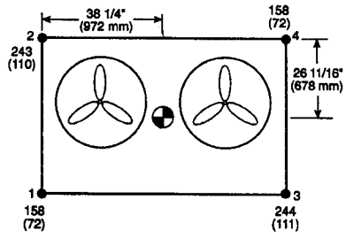
WEIGHT DISTRIBUTION
