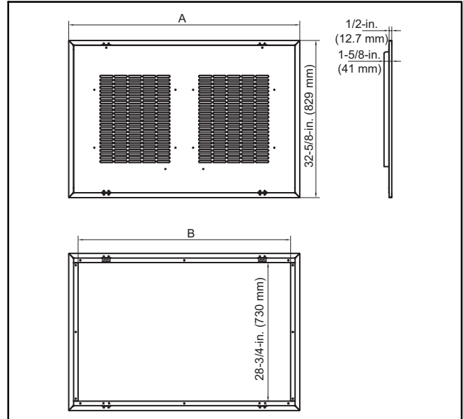
Panel Dimensions, inches (mm)
