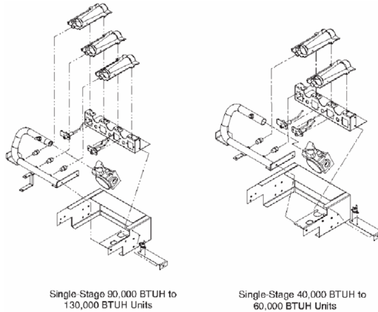
Orifice Installation
