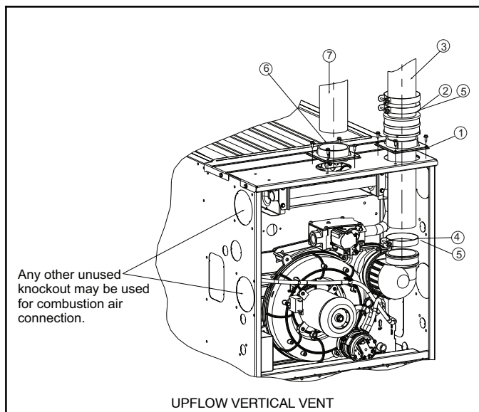
Figure 44 - Upflow Configurations (Appearance may vary) See "Notes for Venting Options"
