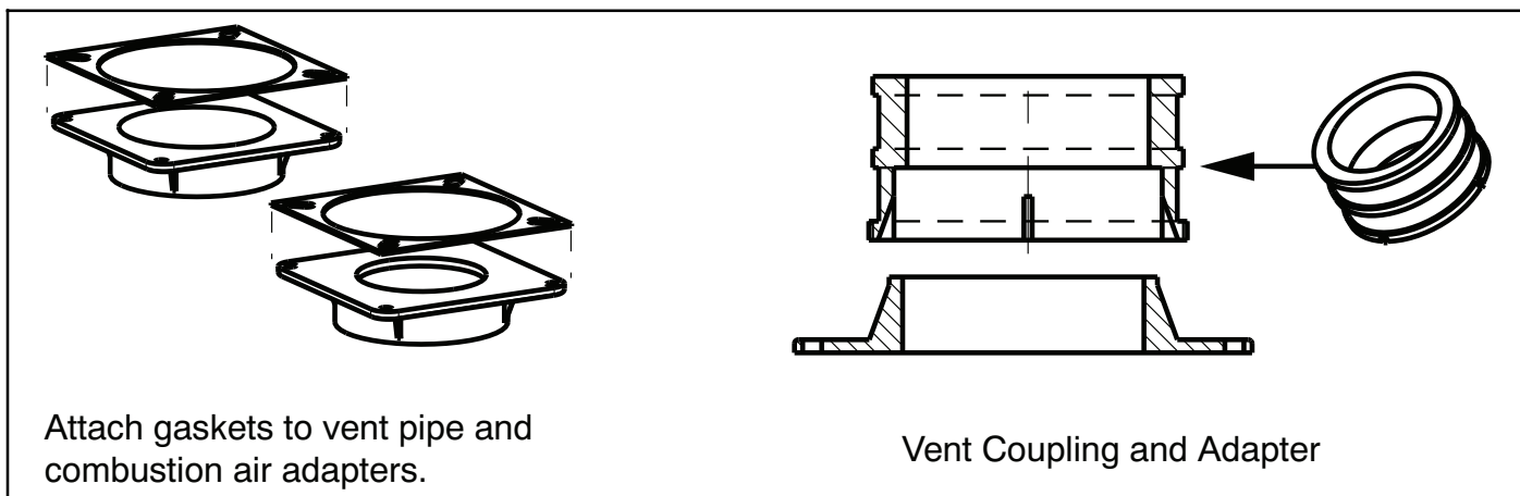
Figure 41 - Vent Coupling and Adapter with Gaskets
