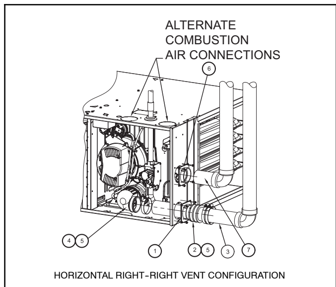
Figure 47 - Horizontal Right (Appearance may vary) See "Notes for Venting Options"
