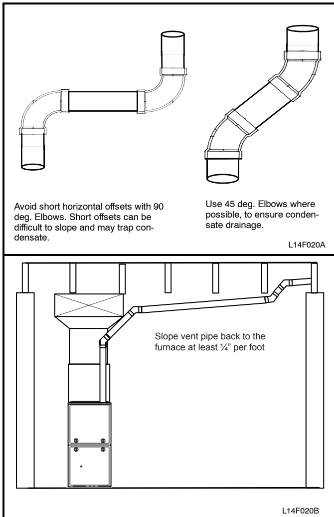
Figure 40 - Combustion-Air and Vent Pipe Diameter Transition Location and Elbow Configuration
