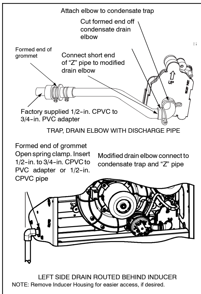
Figure 18 - Drain Trap Connection and Routing (Appearance May Vary)
