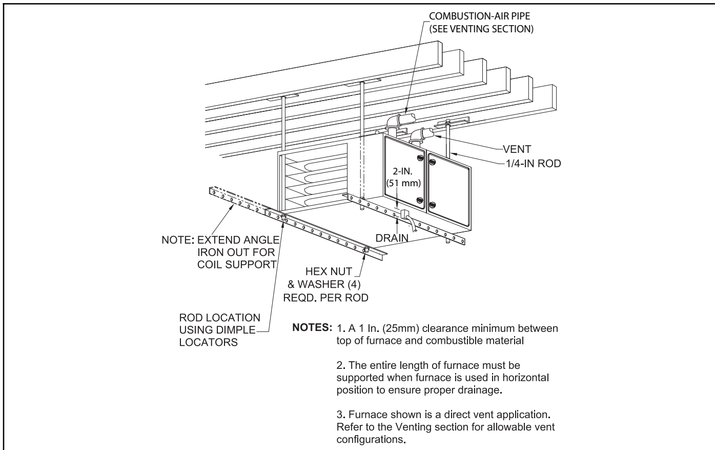
Figure 30 - Suspended Furnace Installation
