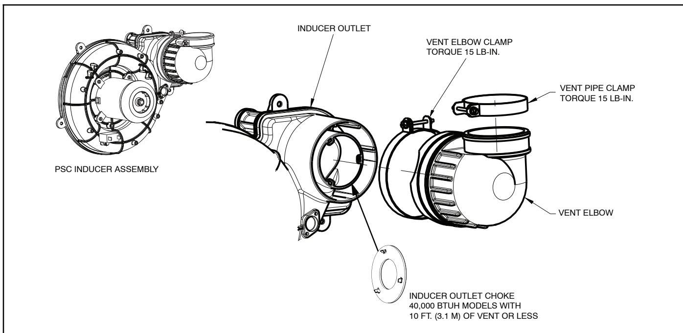
Figure 42 - Inducer Vent Elbow
