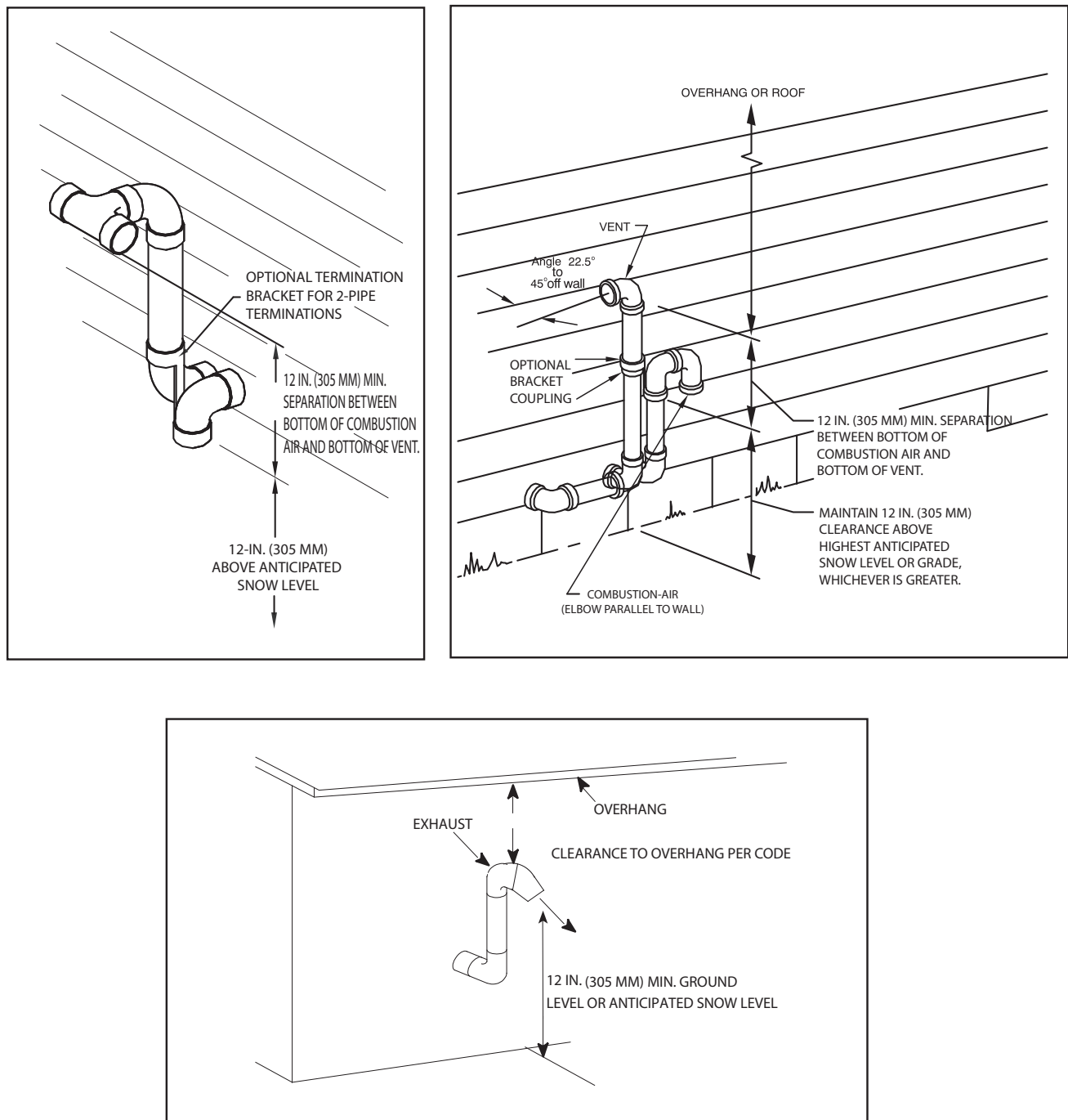
Figure 54 - Alberta and Saskatchewan Vent Termination
