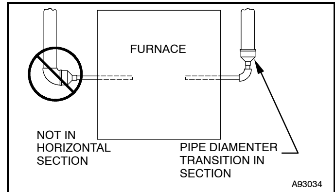
Figure 39 - Combustion-Air and Vent Pipe Diameter Transition Location and Elbow Configuration
