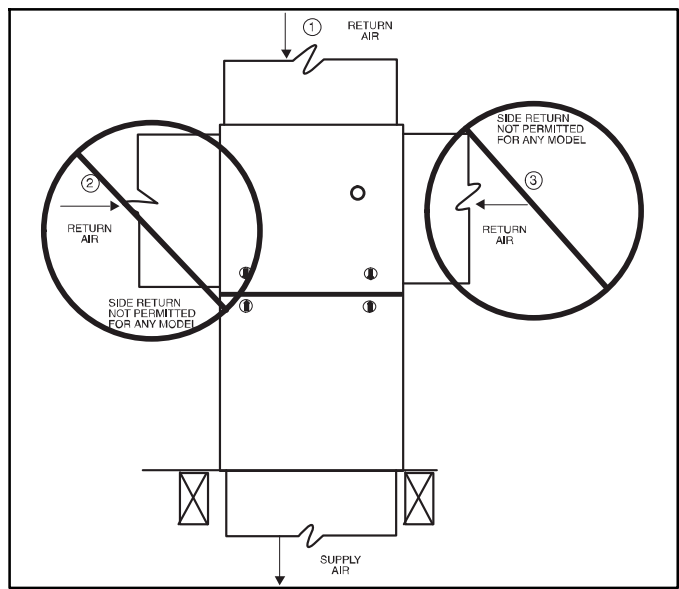
Figure 27 - Downflow Return Air Configurations and Restrictions
