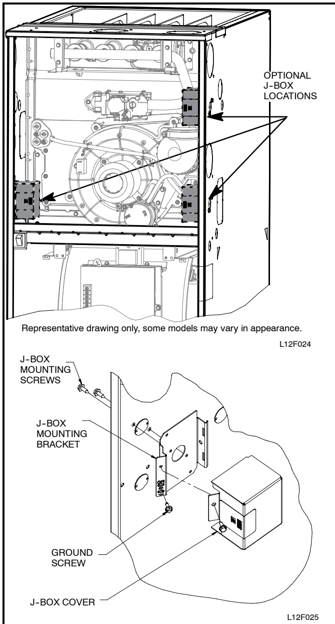
Figure 34 - Installing J-Box (When Used)
