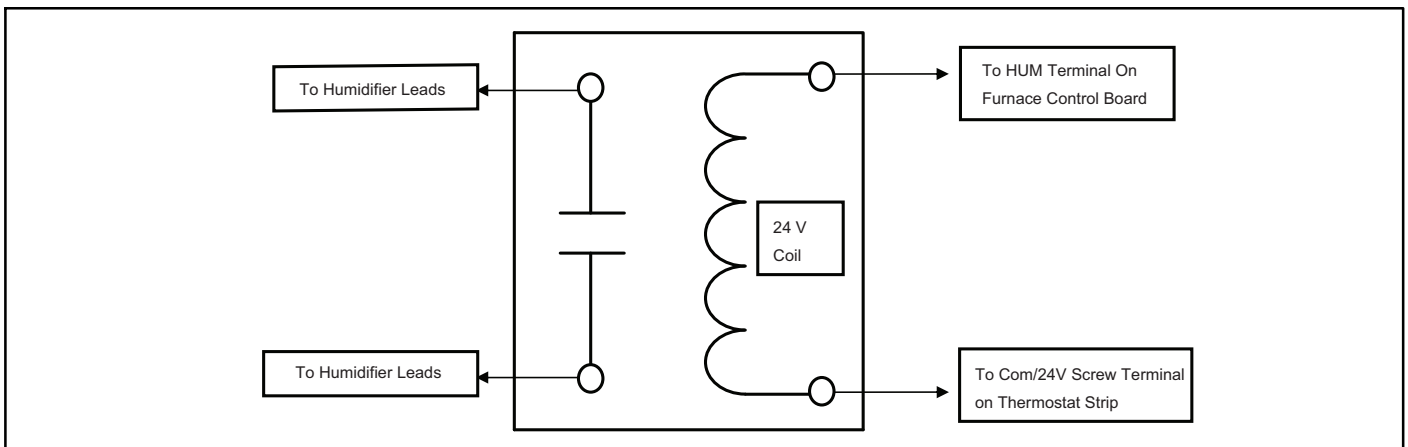
Figure 36 - Field-supplied Isolation Relay for Humidifiers with Internal Power Supply
