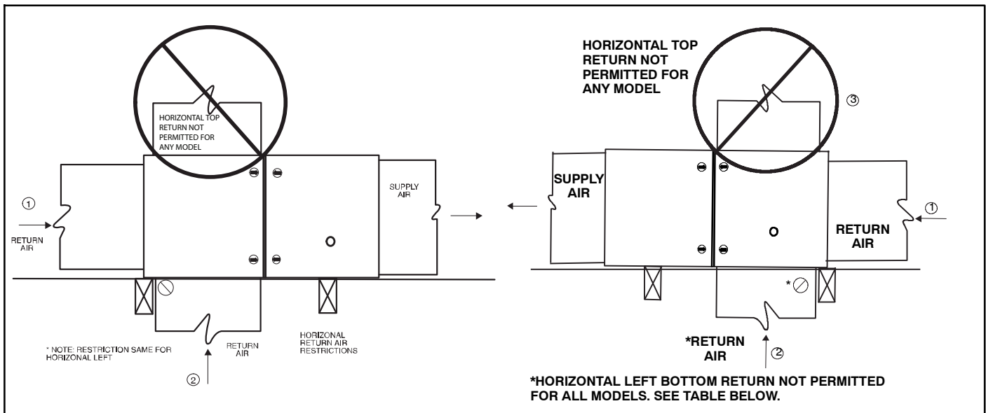
Figure 28 - Horizontal Return Air Configurations and Restrictions
