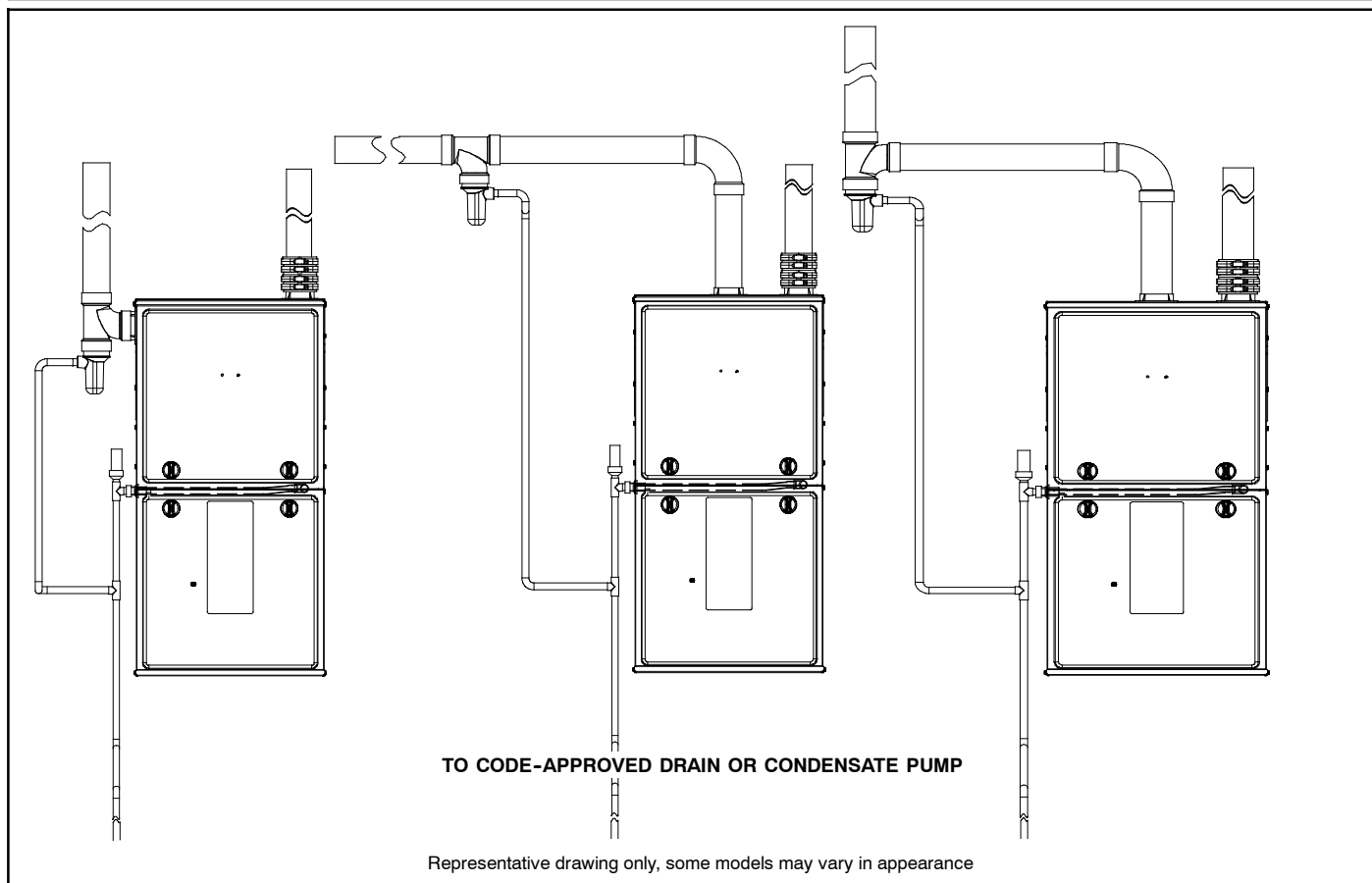
Figure 56 - Recommended Combustion Air Inlet Moisture Trap
