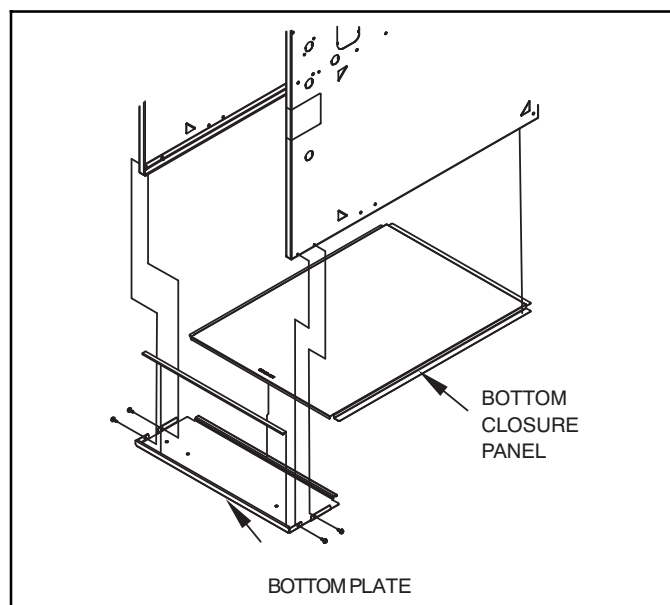
Figure 24 - Removing Bottom Closure Panel
