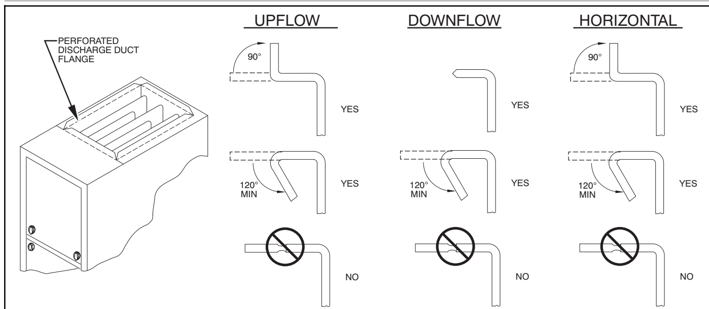
Figure 22 - Duct Flanges
