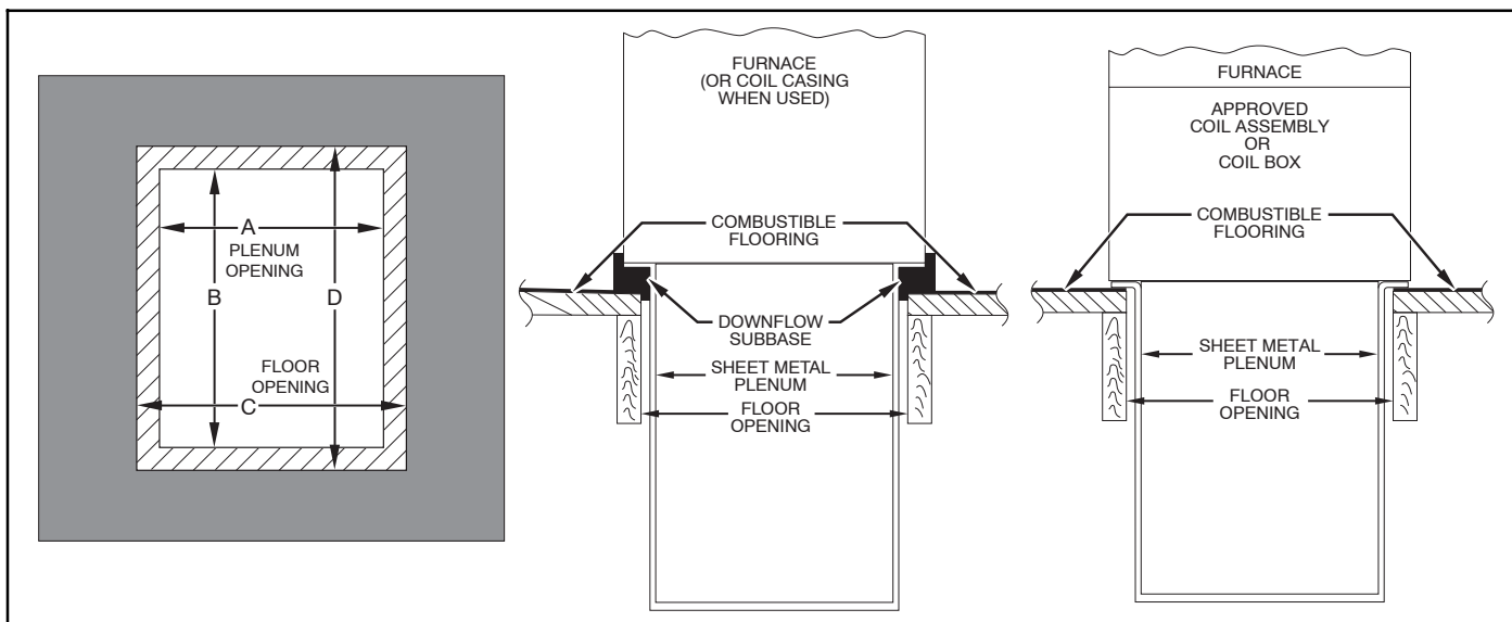
Figure 21 - Installation on Combustible Flooring
