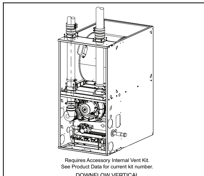
Figure 45 - Downflow Configurations (Appearance may vary) See "Notes for Venting Options"
