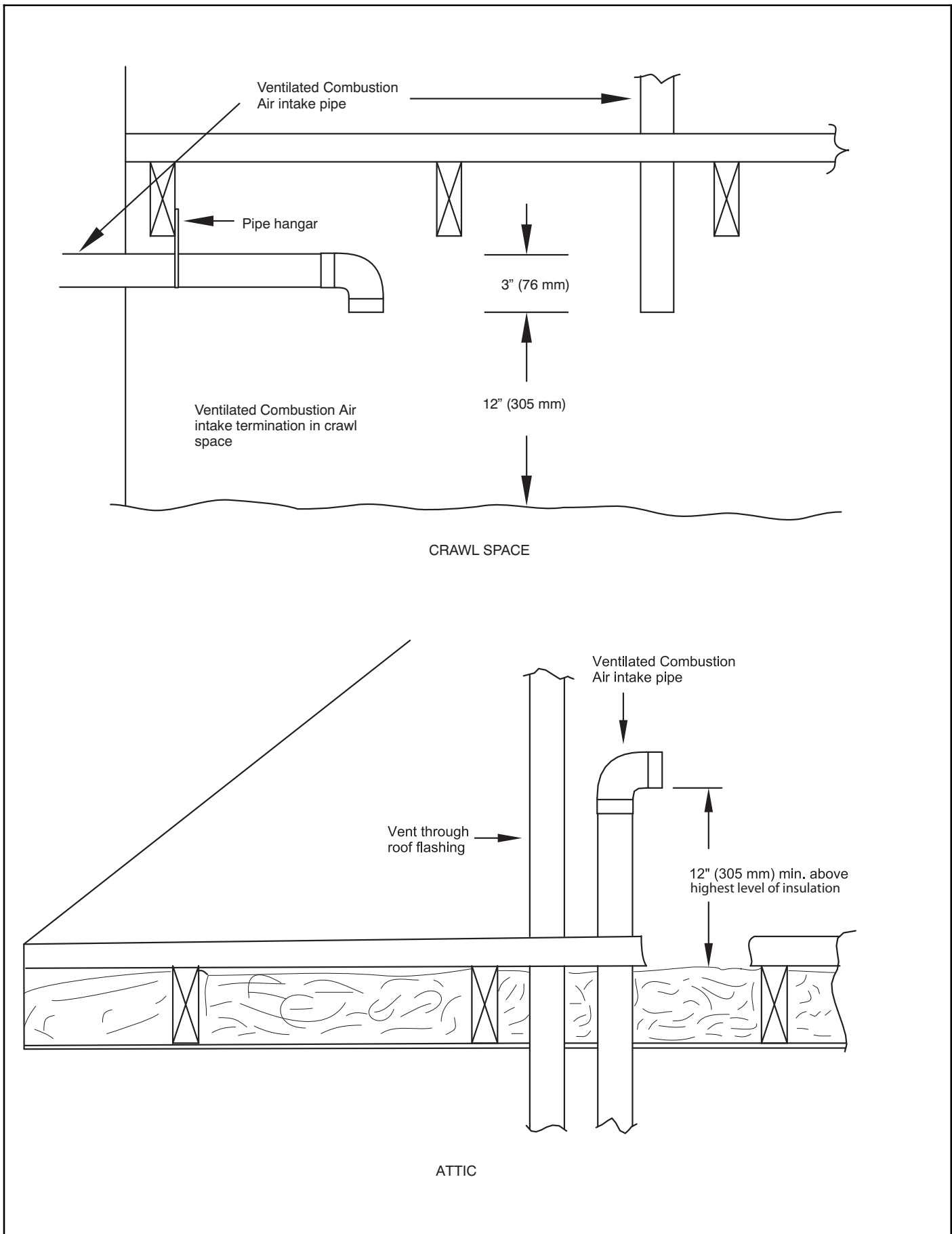
Figure 55 - Vent Terminations for Ventilated Combustion Air
