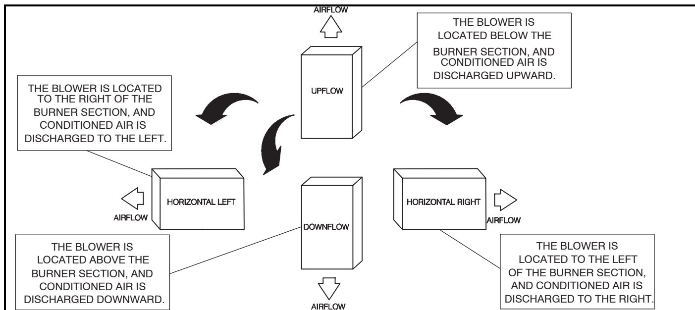
Figure 2 - Multipoise Orientations
