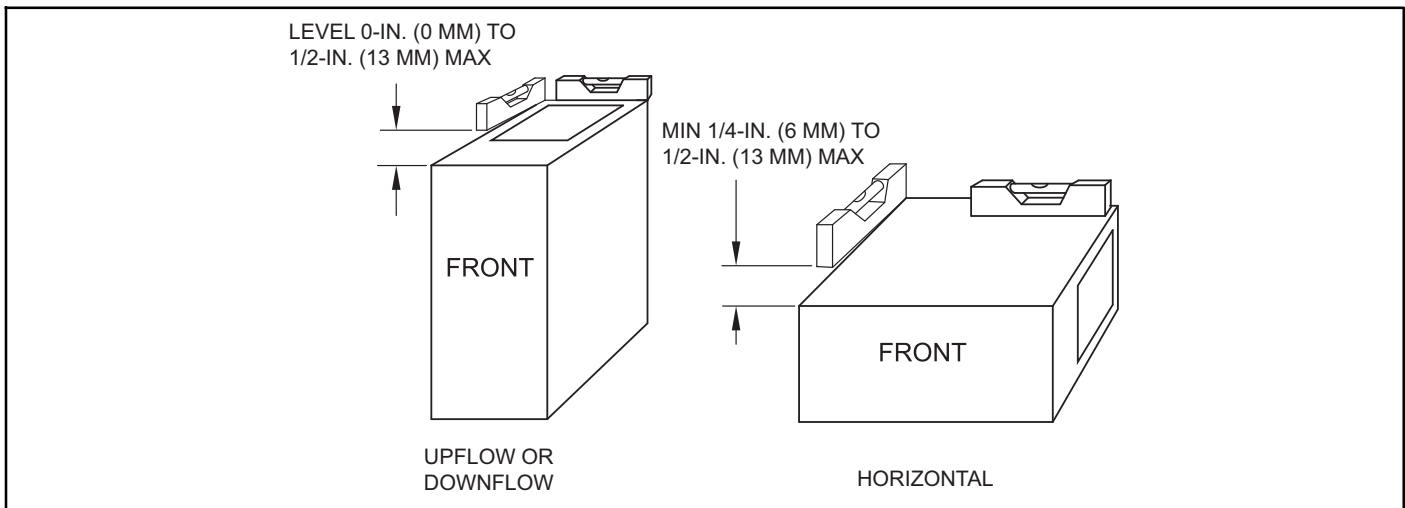
Figure 25 - Furnace Pitch Requirements
