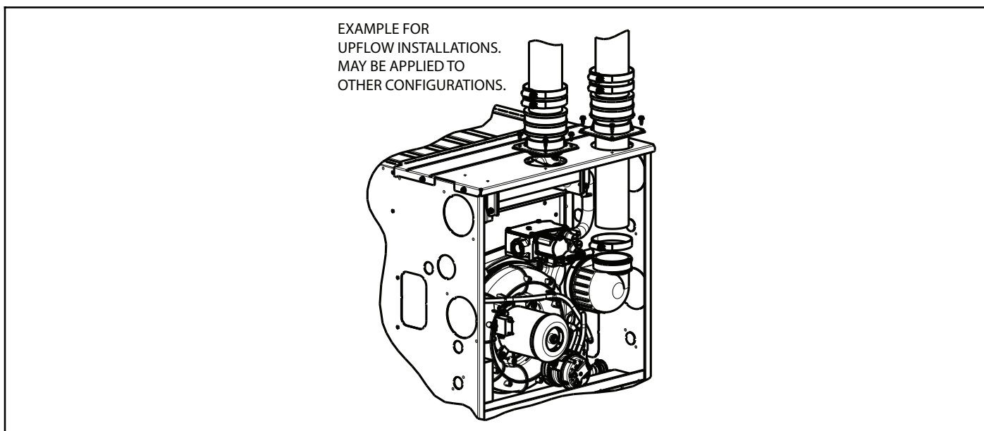
Figure 43 - Sample Inlet Air Pipe Connection for Polypropylene Venting Systems
