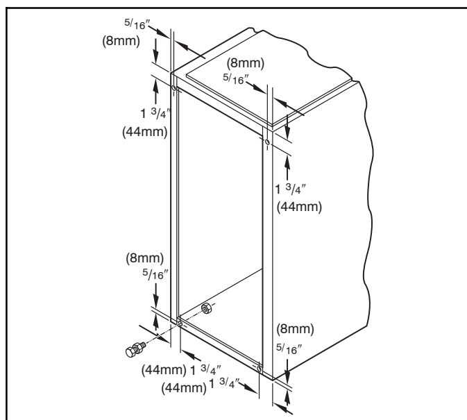
Figure 23 - Leveling Legs
