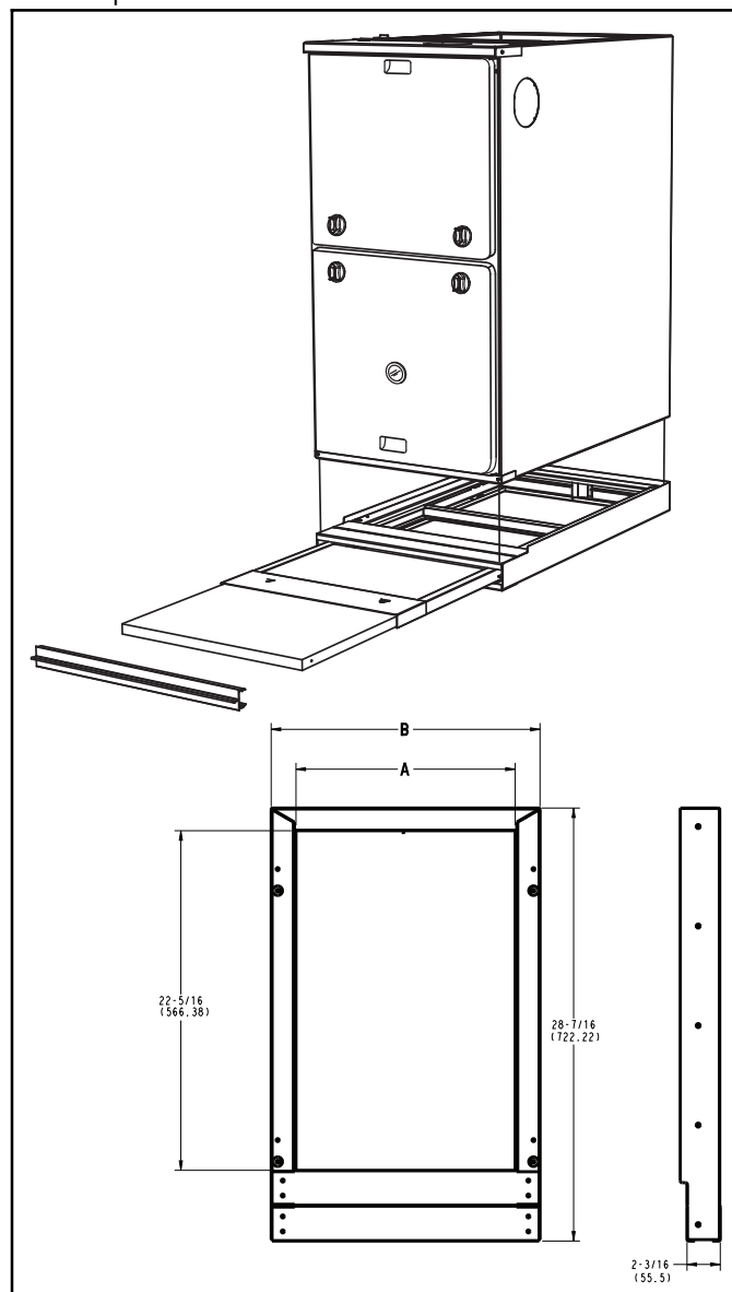
Figure 20 - Accessory Bottom Filter
