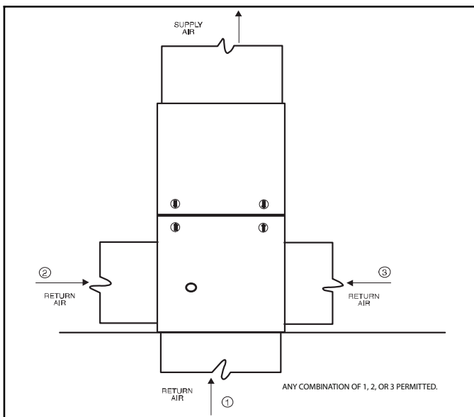
Figure 26 - Upflow Return Air Configurations and Restrictions
