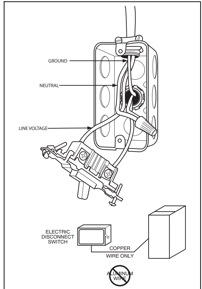
Figure 35 - Field-Supplied Electrical Box on Furnace Casing
