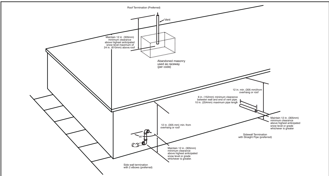
Figure 53 - Vent Pipe Termination for Non-Direct Vent and Ventilated Combustion Air System
