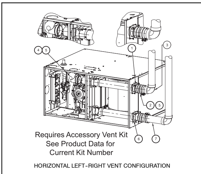
Figure 46 - Horizontal Left (Appearance may vary) See "Notes for Venting Options"
