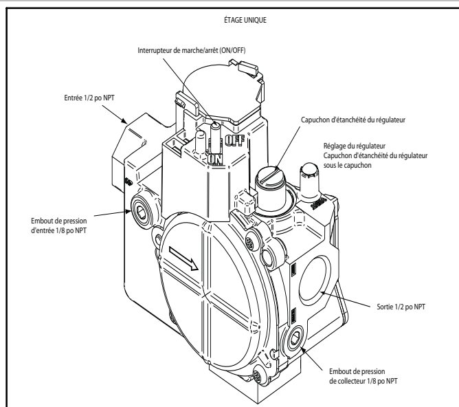
Figure 30 – Vanne de gaz
