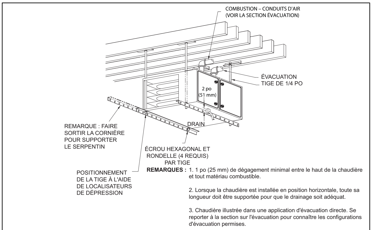
Figure 29 – Installation de chaudière suspendue
