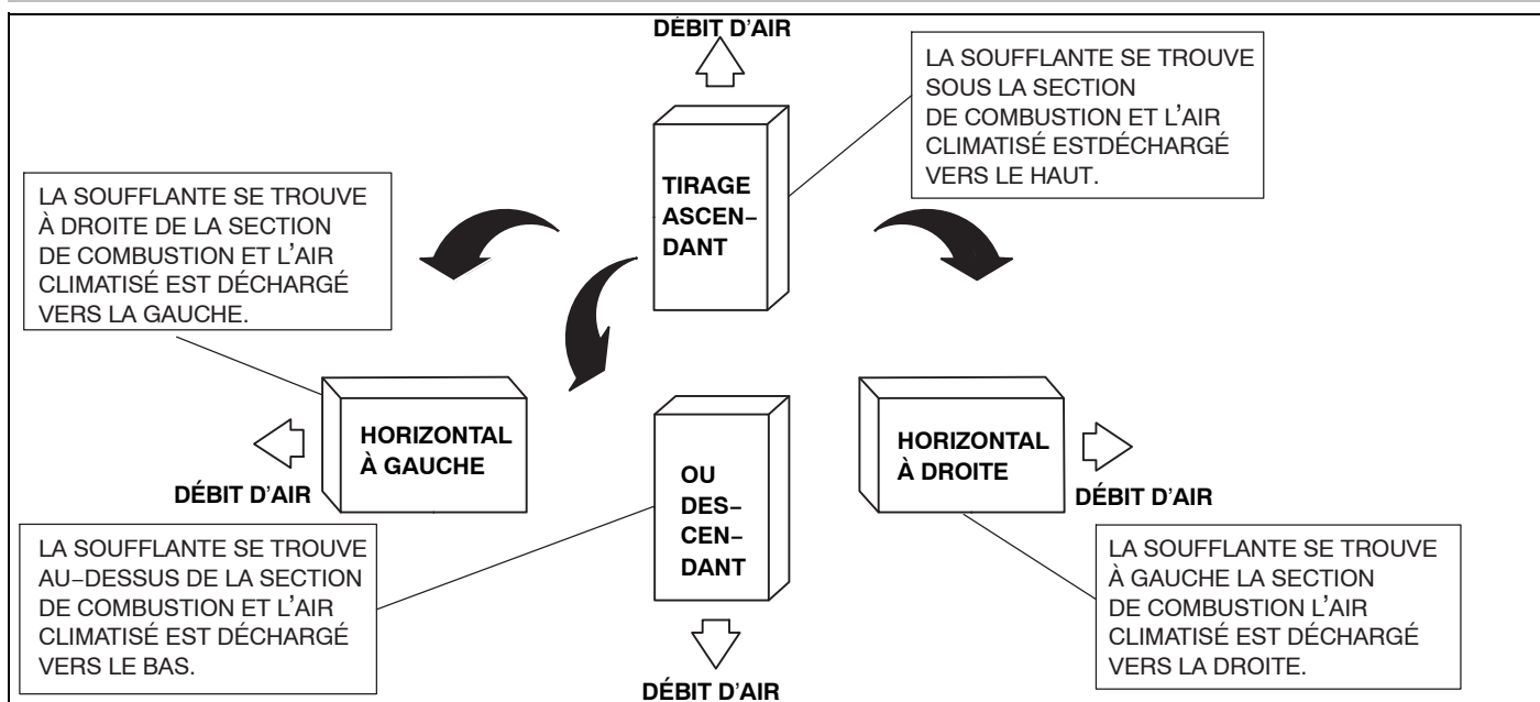
Figure 2 – Orientations à configuration multiple
