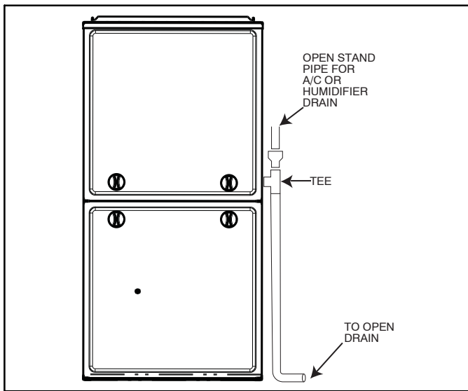
Figure 13 – Example of Field Drain Attachment
