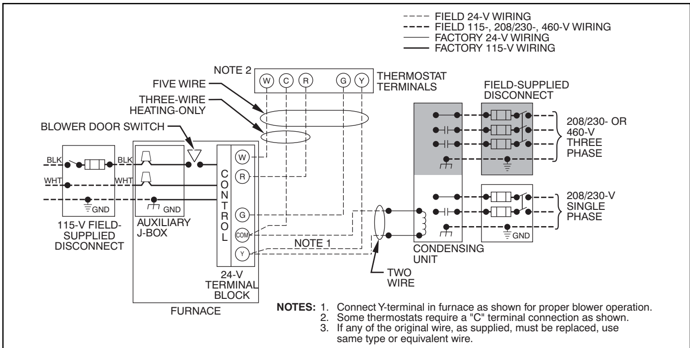
Figure 36 – Typical Single-Stage Wiring Diagram
