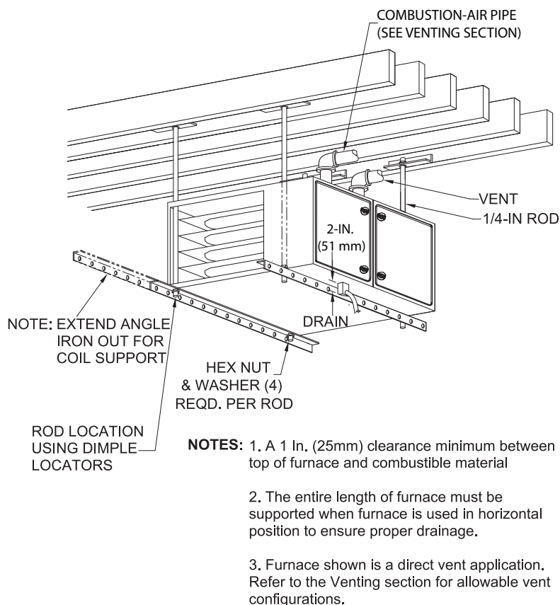
Figure 29 – Suspended Furnace Installation
