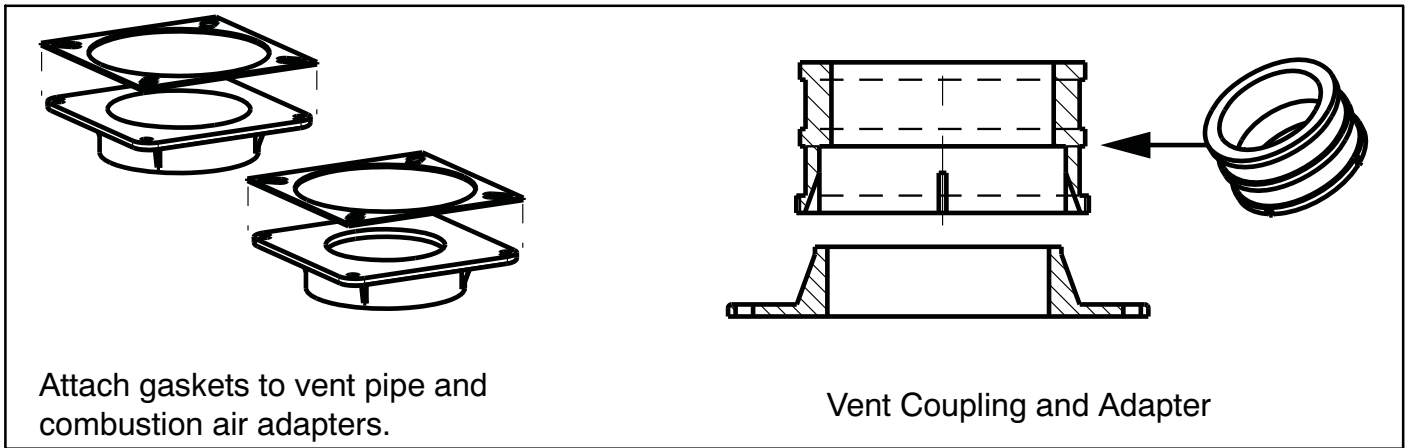
Figure 38 – Vent Coupling and Adapter with Gaskets
