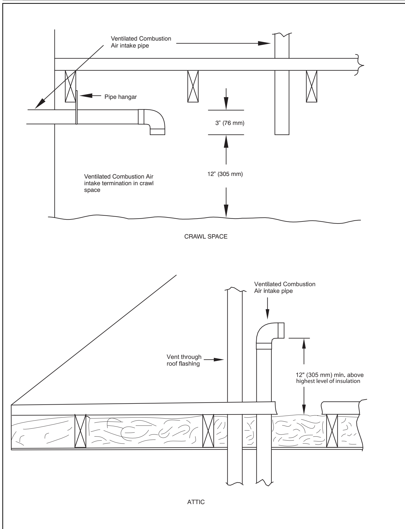
Figure 52 – Vent Terminations for Ventilated Combustion Air
