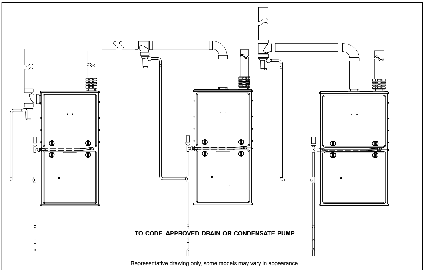
Figure 53 – Optional Combustion Air Inlet Moisture Trap
