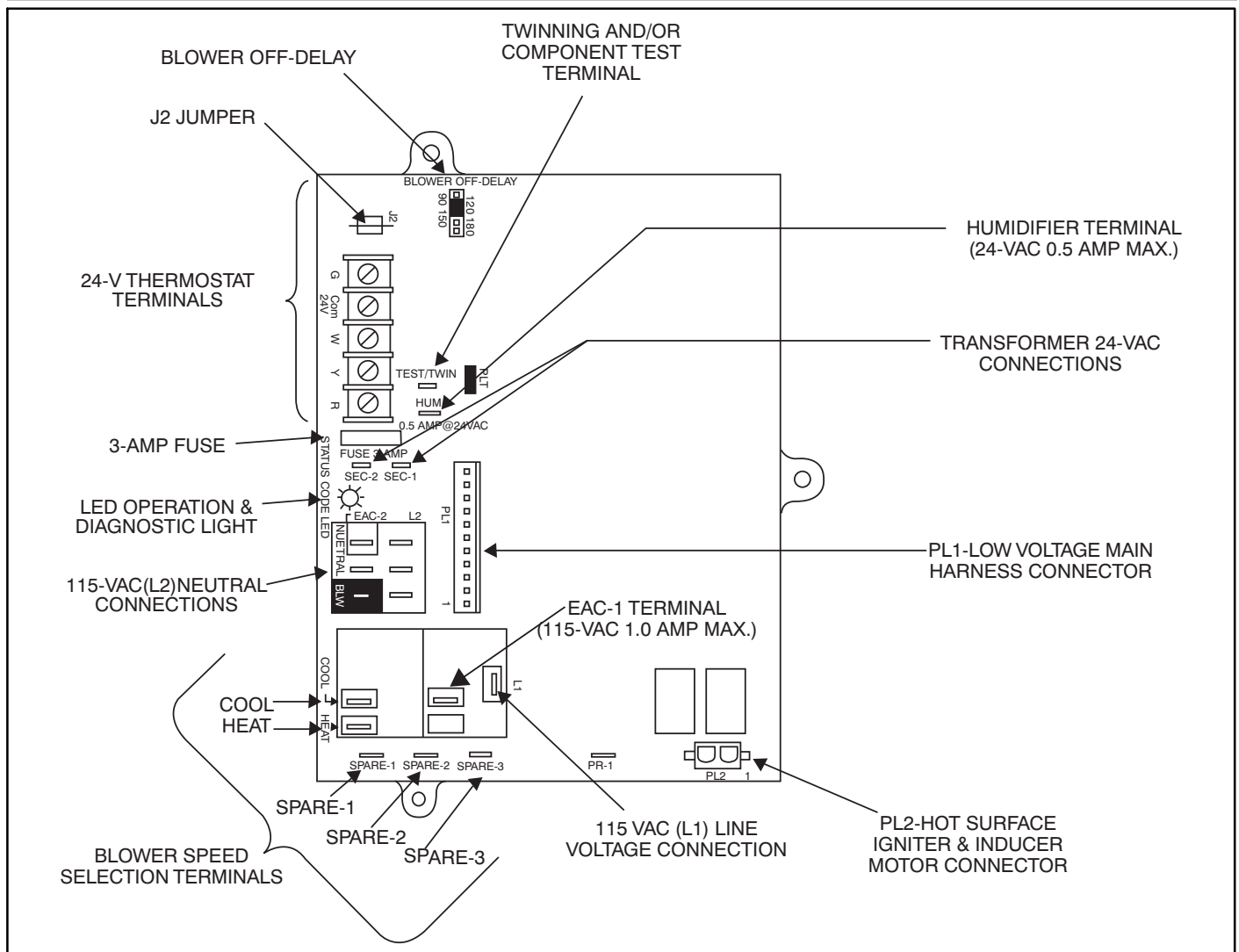
Figure 37 – Example of Single Stage Furnace Control
