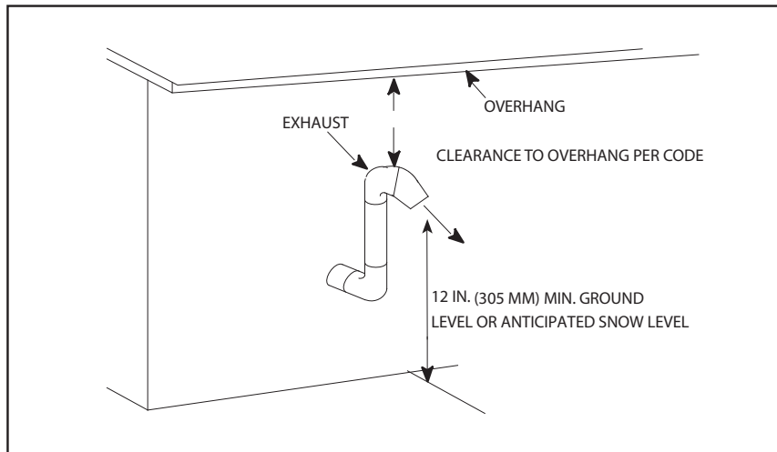
Figure 51 – Alberta and Saskatchewan Vent Termination
