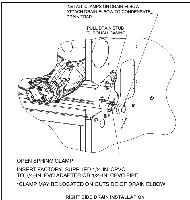
Figure 13 – Example of Field Drain Attachment
