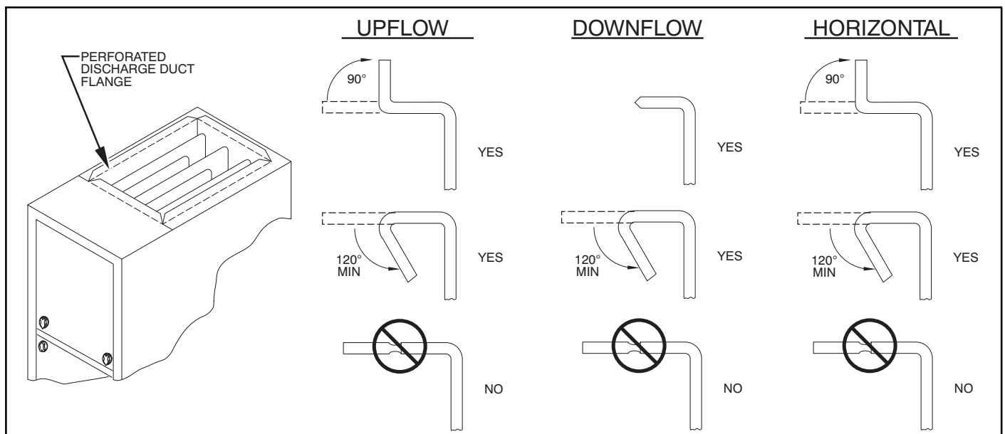
Figure 21 – Duct Flanges
