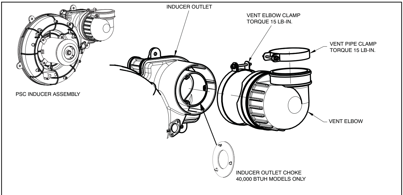
Figure 39 – Inducer Vent Elbow
