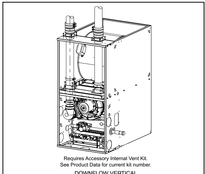
Figure 42 – Downflow Configurations (Appearance may vary) See “Notes for Venting Options”
