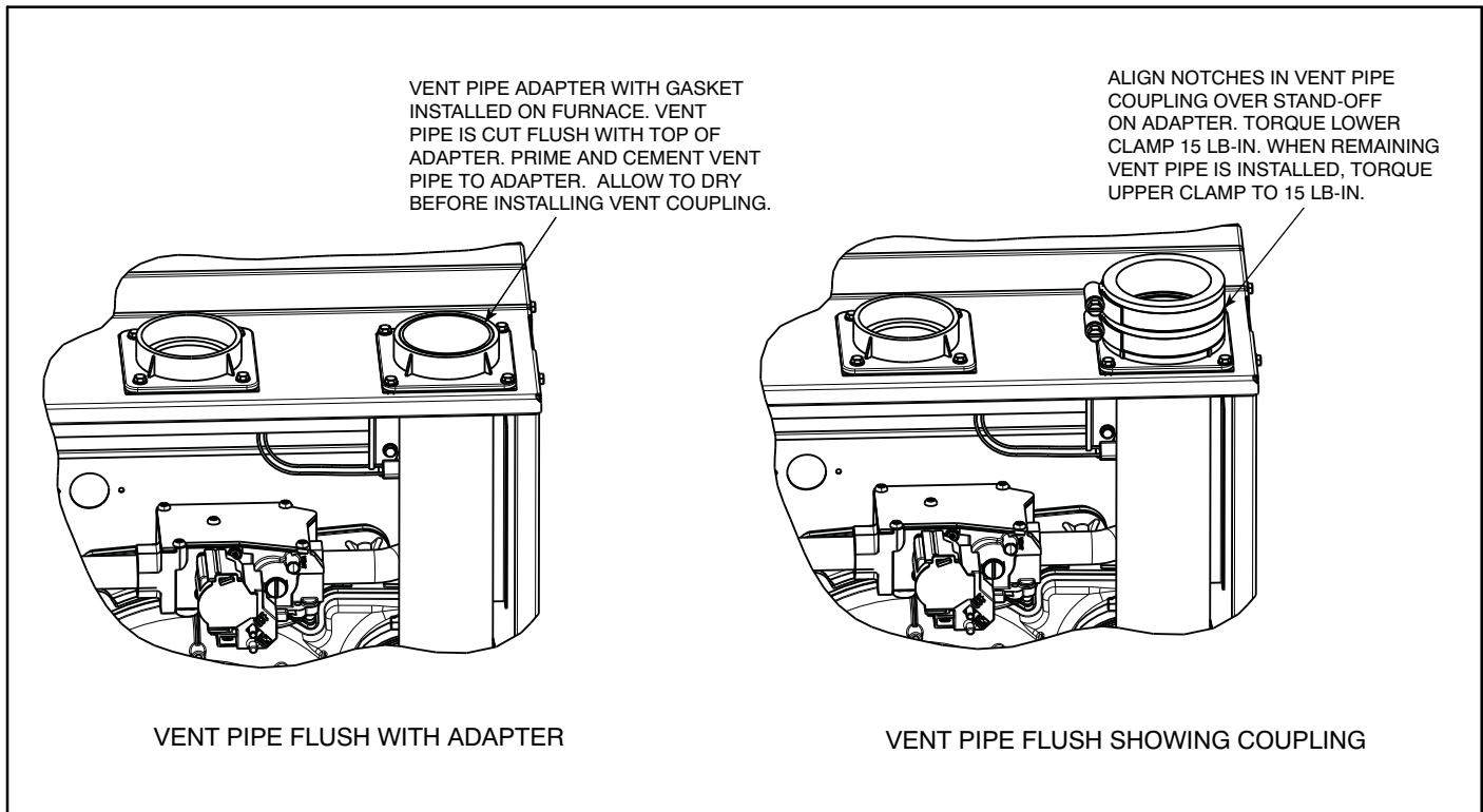
Figure 45 – Vent Pipe Flush with Adaptor
