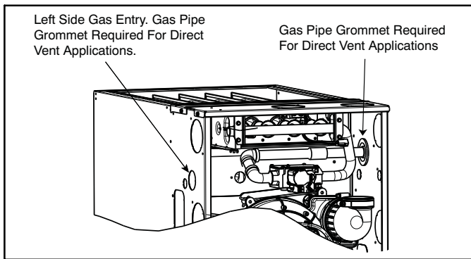
Figure 31 – Gas Entry
