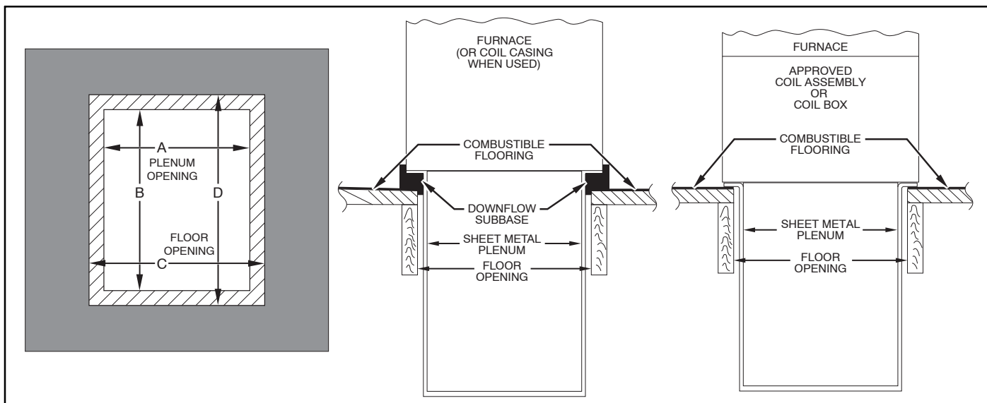
Figure 20 – Installation on Combustible Flooring
