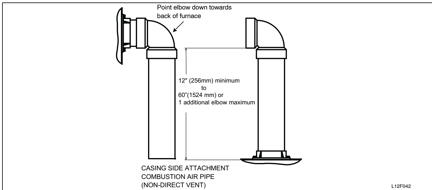
Figure 46 – Combustion Air Pipe Attachment
