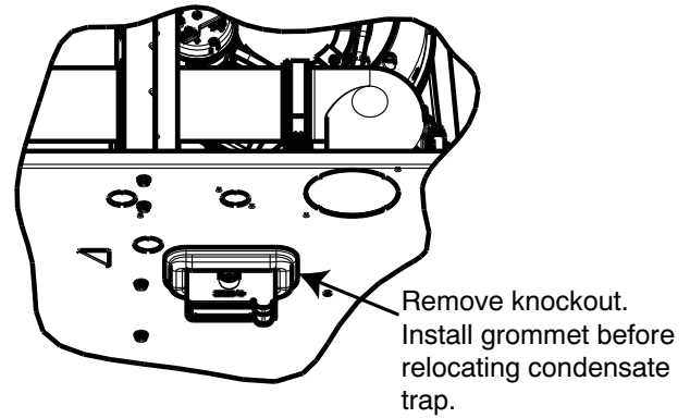
Figure 16 – Accessory Horizontal Drain Trap Grommet
