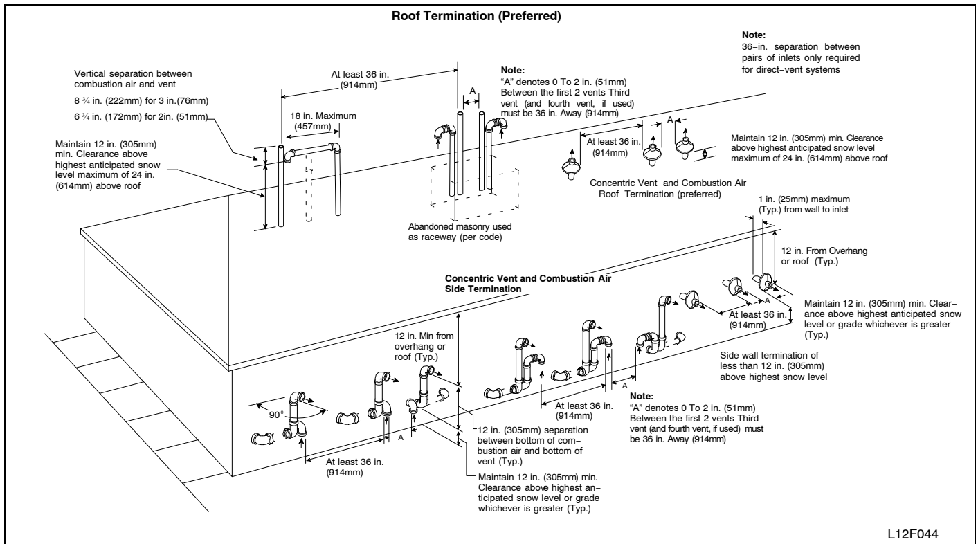
Figure 49 – Combustion Air and Vent Pipe Termination for Direct Vent (2-Pipe) System
