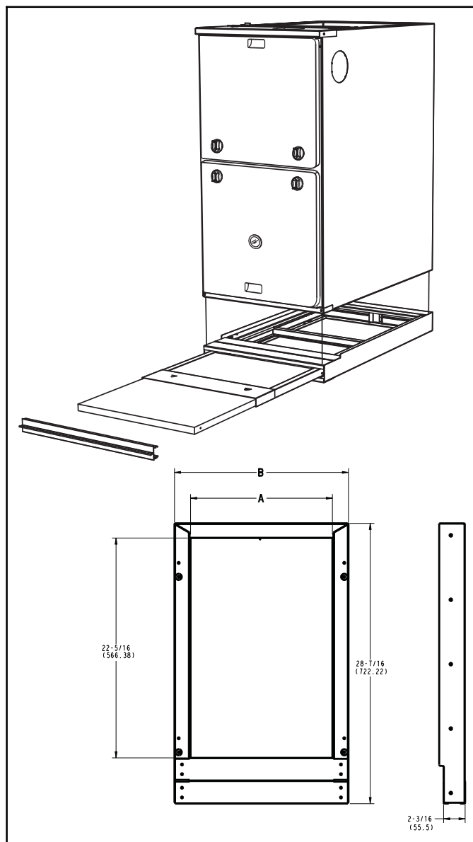
Figure 19 – Accessory Bottom Filter
