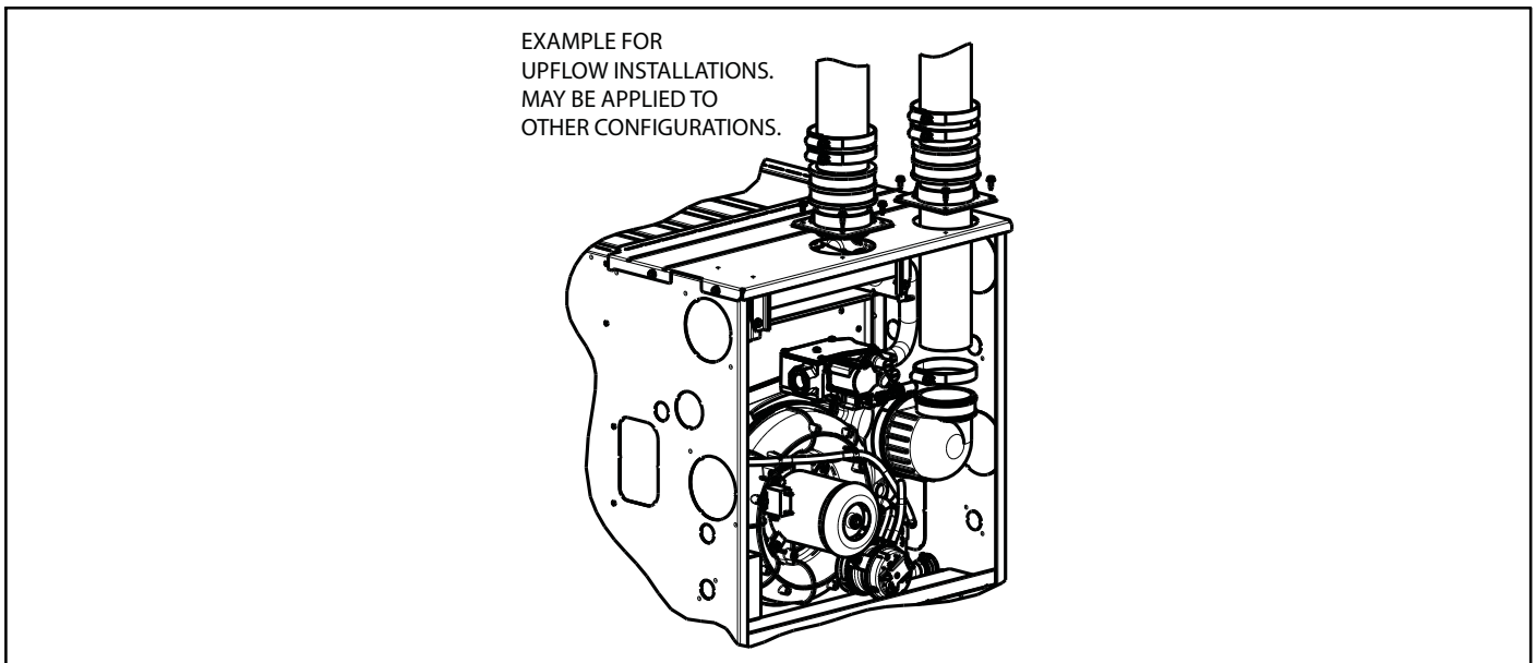
Figure 40 – Sample Inlet Air Pipe Connection for Polypropylene Venting Systems
