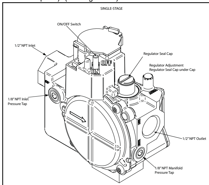
Figure 30 – Gas Valve
