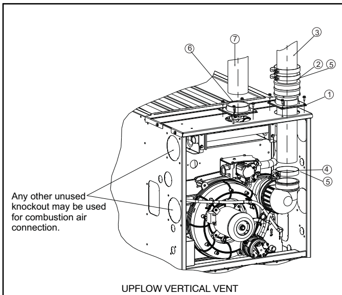
Figure 41 – Upflow Configurations (Appearance may vary) See “Notes for Venting Options”
