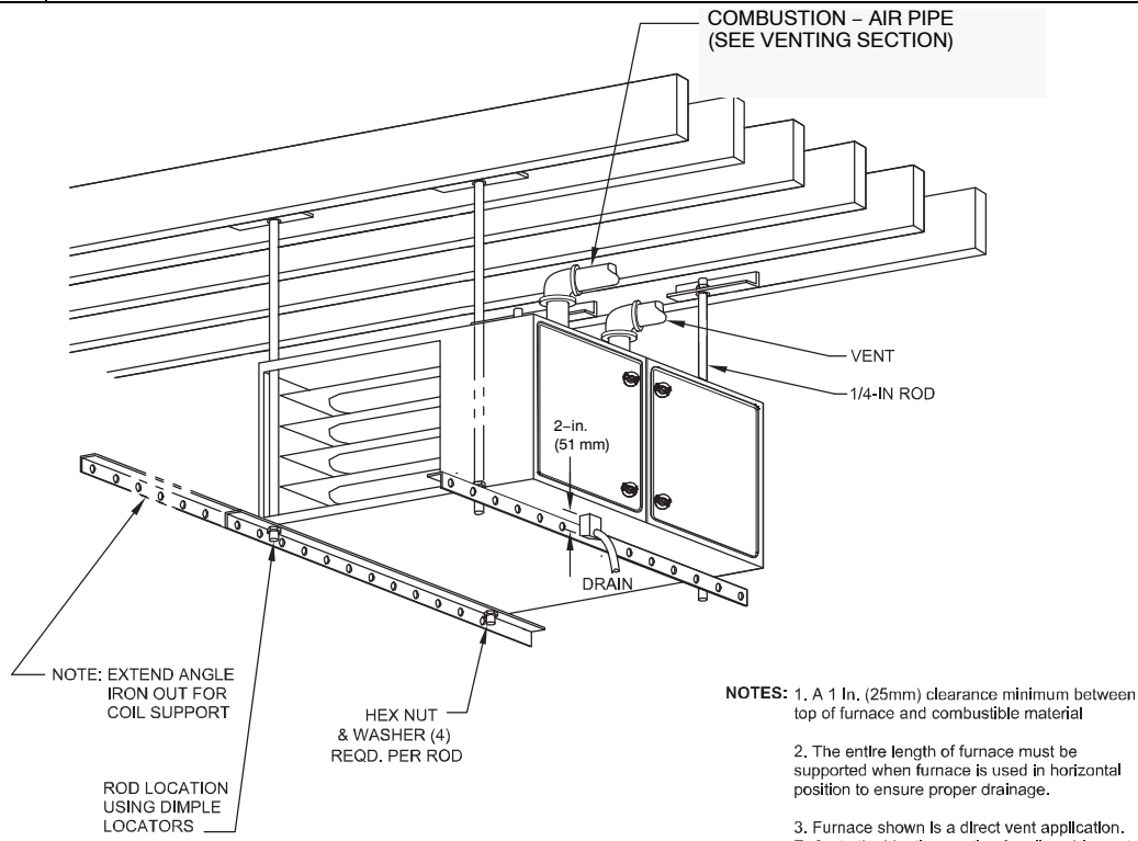
Figure 25 Suspended Furnace Installation
