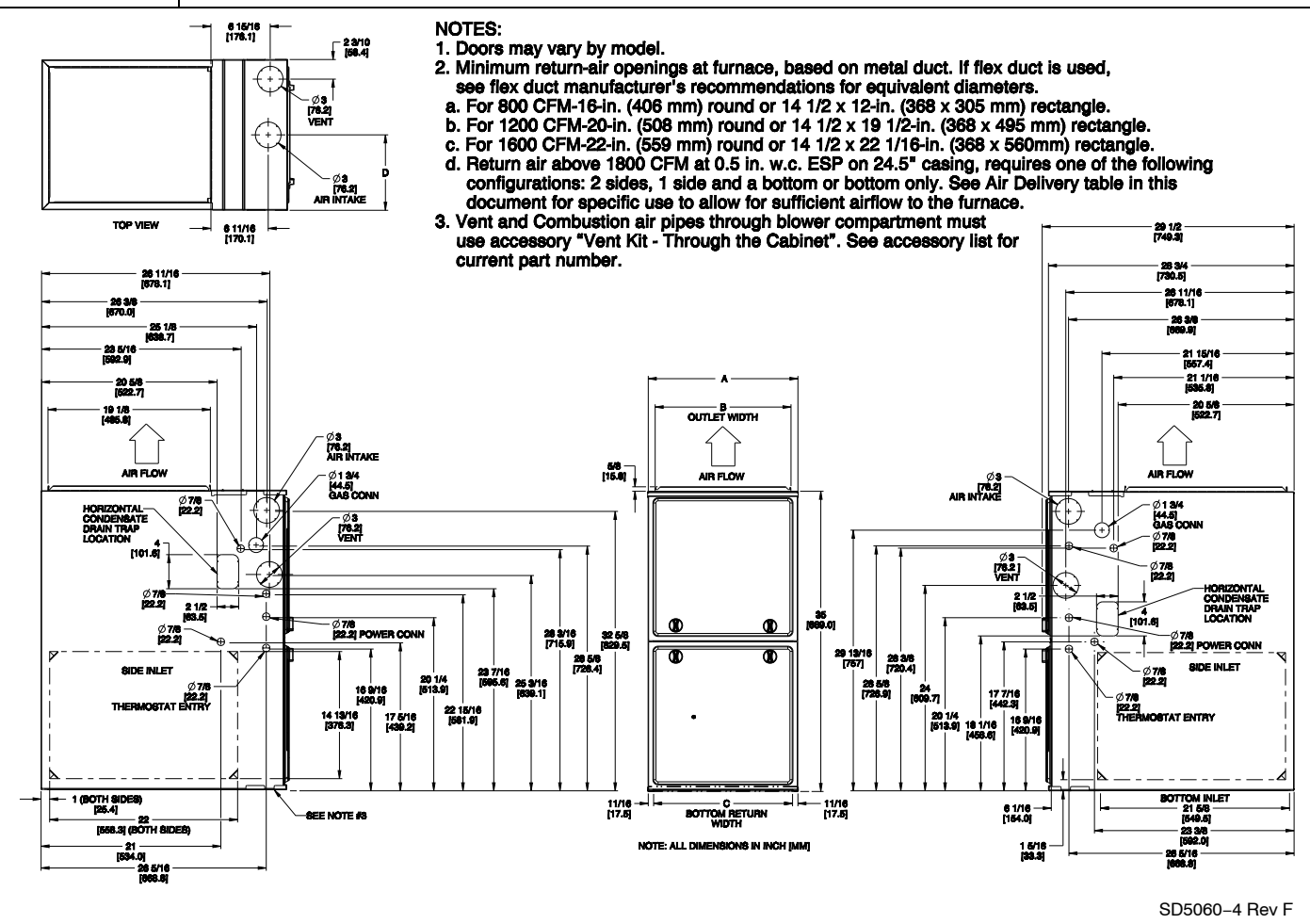
Figure 2 Dimensions
